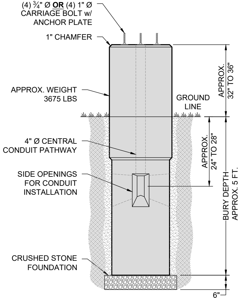
INSTALLED PRODUCT VIEW SCALE: 1/2" = 1'-0"
