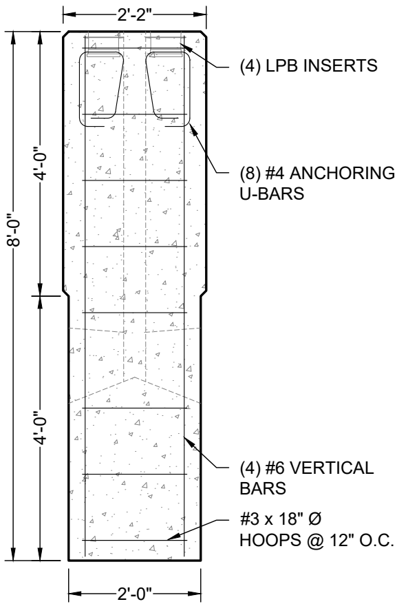
PRODUCT SECTION VIEW SCALE: 1/2" = 1'-0"
