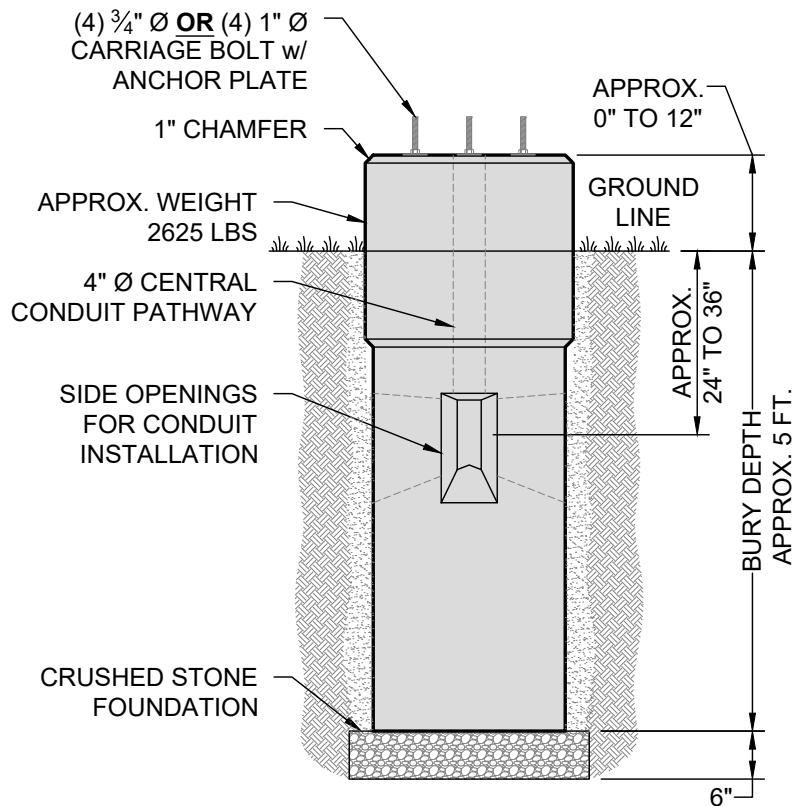
INSTALLED PRODUCT VIEW SCALE: 1/2" = 1'-0"
